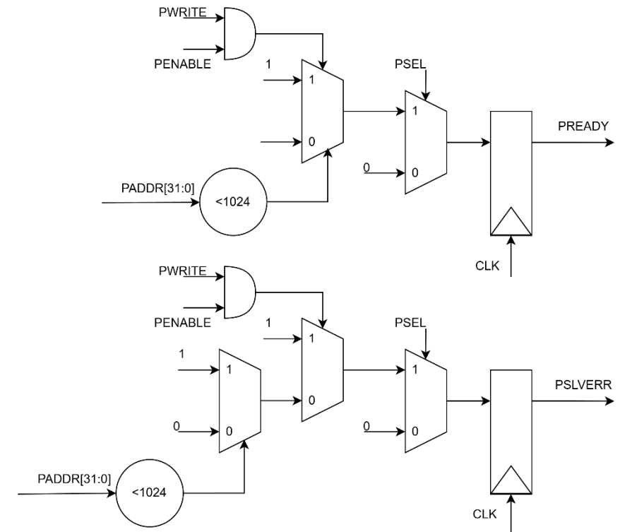
APB Slave Output signals
