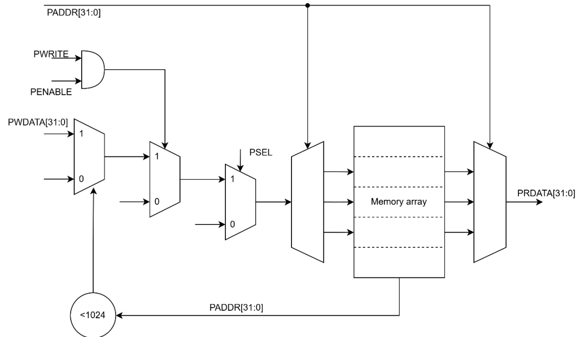
APB Slave RAM
